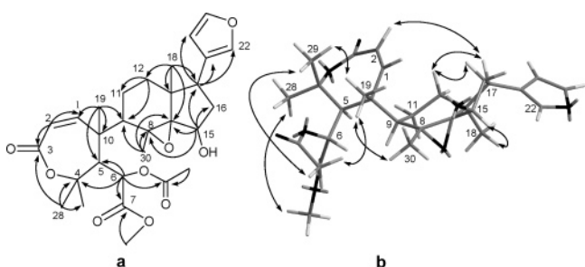
Figure 4. Selected HMBC (H-C) (a) and NOESY ( \leftrightarrow ) (b) correlations of toonaciliatin E (5).
