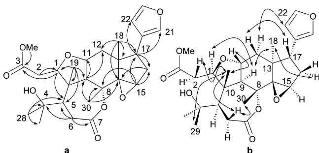
Figure 3. Selected HMBC (H-C) (a) and NOESY ( \leftrightarrow ) (b) correlations of toonaciliatin D (4).
